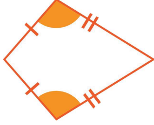
kite
