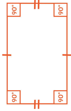
rectangle
