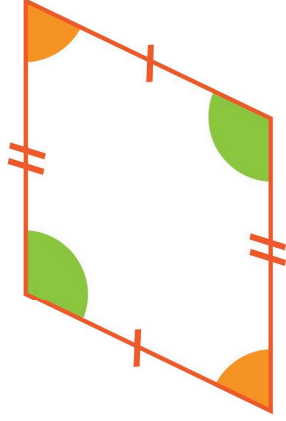
parallelogram
